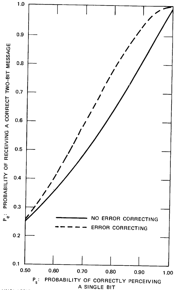
FIGURE D-1 USE OF A 5-BIT ERROR-CORRECTING CODE TO INCREASE PROBABILITY OF CORRECT MESSAGE RECEPTION (U)
